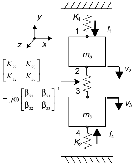
Figure 7. Discrete model of physical system used to examine approximate methods.
