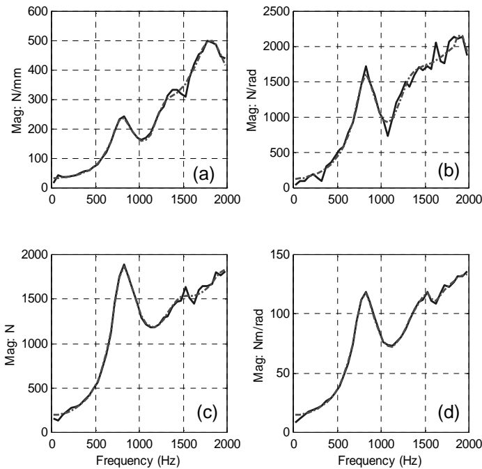
Figure 13. Transfer stiffnesses in flexural motion for isolator, as extracted using the identification scheme. (a) Lateral stiffness modulus; (b) coupling stiffness modulus; (c) coupling stiffness modulus; (d) rotational stiffness. Key: —, Experimental result; ----, curve fit.
