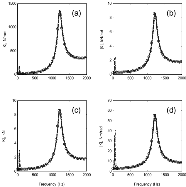
Figure 9. Decomposed flexural stiffnesses for symmetric beam of Figure 3(c) using a system consisting of two rigid masses and an elastic beam as shown in Figure 3(b). (a) Force stiffness; (b) coupling stiffness; (c) coupling stiffness; (d) moment stiffness. Key: —, Mobility synthesis method; ----, approximate method using equation (20b); -.-.-, approximate method using equation (21b); o, direct analytical solution.
