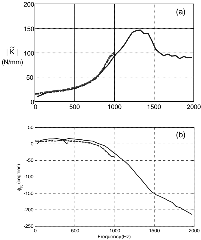
Figure 12. Comparison of axial dynamic stiffnesses for isolator. (a) Dynamic stiffness modulus; (b) loss angle. Key: —, Mobility model; ----, Measured (MTS): f_{\text{mean}} = 3 N; - - - , Measured (MTS): f_{\text{mean}} = 12 N; ..... , Measured (MTS): f_{\text{mean}} = 23 N.
