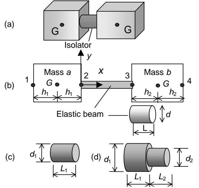
Figure 3. Proposed identification scheme. (a) Schematic; (b) simulation example; (c) symmetric isolator used for simulation; (d) asymmetric isolator used for simulation.
