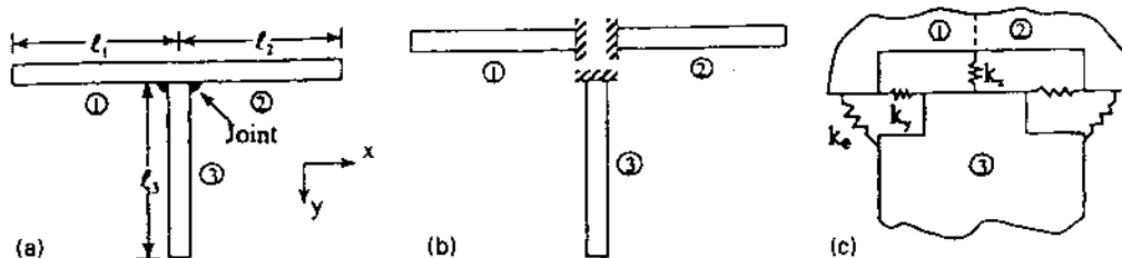
Figure 7. "T" beam assembly and synthesis approach. (a) Schematic, (b) component synthesis for an ideal joint, (c) joint stiffness matrix model.
