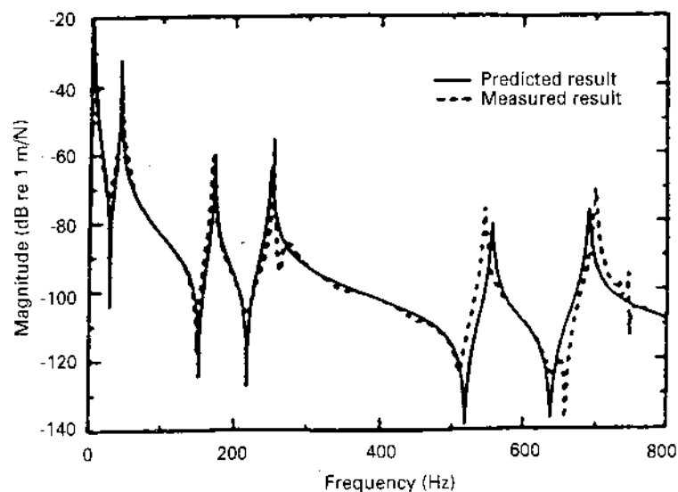
Figure 8. Driving point compliance for "T" beam.
