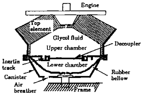
Figure 1. Hydraulic engine mount (passive design).
