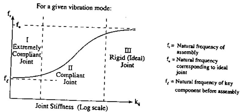
Figure 10. Natural frequency versus joint stiffness relationship depicting three distinct regimes.
