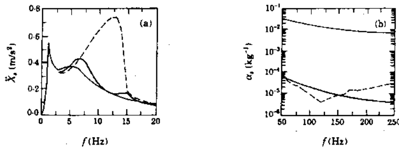
Figure 6. Comparison of passive, adaptive and active mounts. Harmonic responses for three mounting modes in the vehicle model: - - - passive mount; — adaptive mount; — active mount. (a) \ddot{X}_s(\omega) at lower frequencies; (b) \alpha_s(\omega) at higher frequencies.
