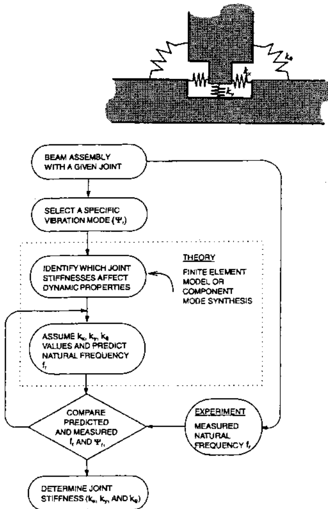
Figure 9. Procedure for estimating the joint stiffness matrix.
