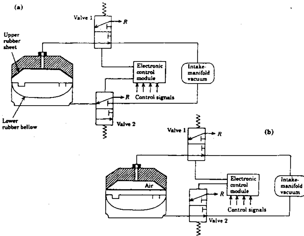
Figure 5. The operation of the proposed adaptive hydraulic mount. Hard, (a) and soft (b) states.
