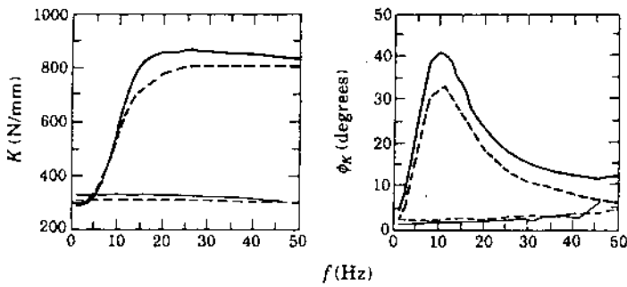
Figure 2. Typical dynamic characteristics of hydraulic mount. Predicted and measured dynamic stiffness spectra of the regular mount. (--- Theory for X = 0.1 mm; — experiment for X = 0.1 mm; --- theory for X = 1.0 mm; — experiment for X = 1.0 mm.)
